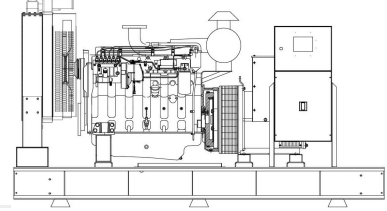
WITHOUT CANOPY
