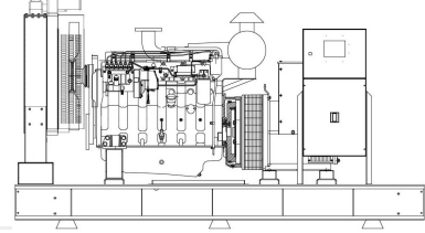
WITHOUT CANOPY
